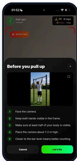
Exercise recognition
